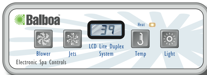
Lite Digital PN 54094 with Overlay PN 10669 • Connects to Main Panel terminal J1
